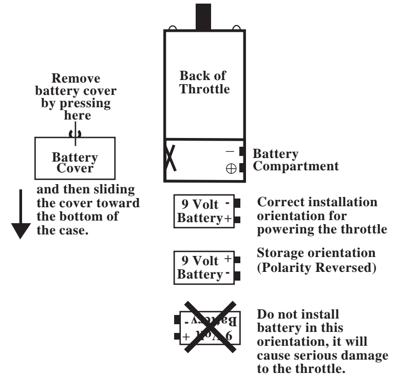
Diagram 4: DT400/R Battery Installation
