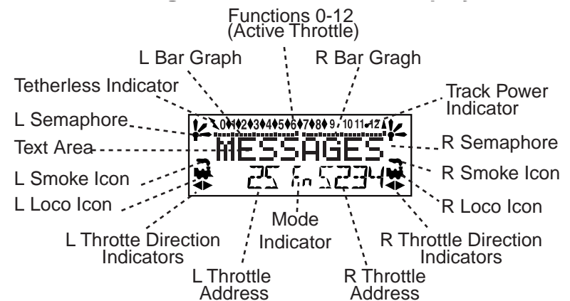
Diagram 3: DT400 LCD
